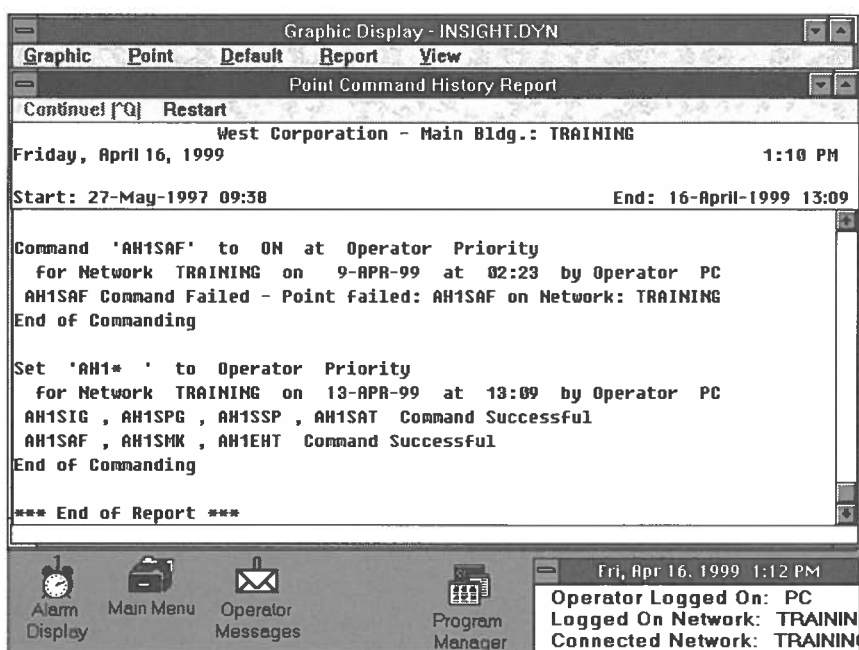
A sample Point Command History report.
