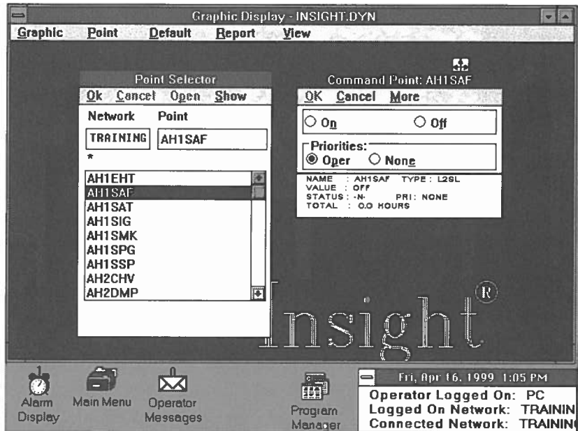
The shortened version of the Command box.
