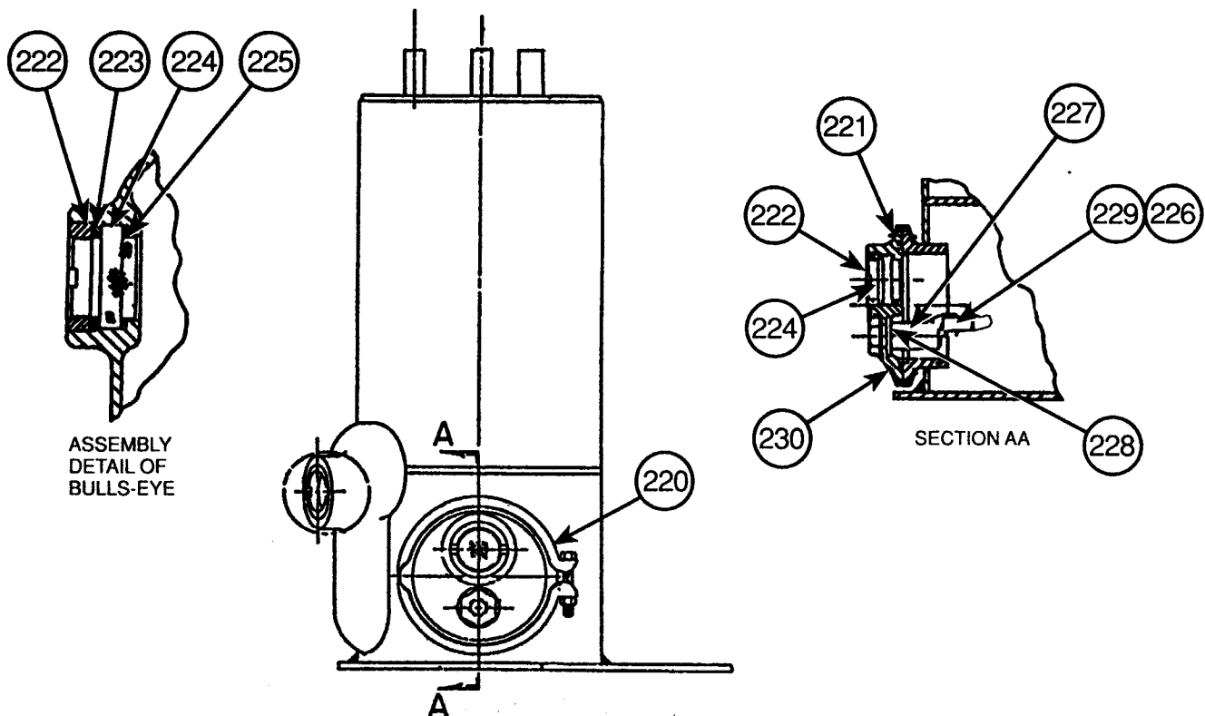
#219-PURGE CONDENSER
