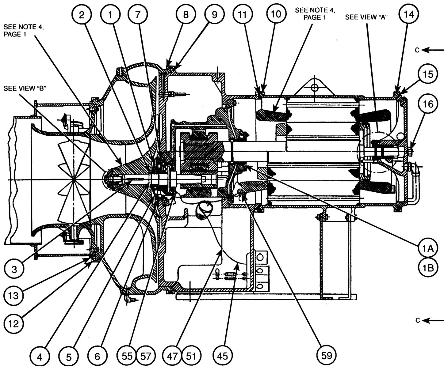
COMPRESSOR ASSEMBLY
